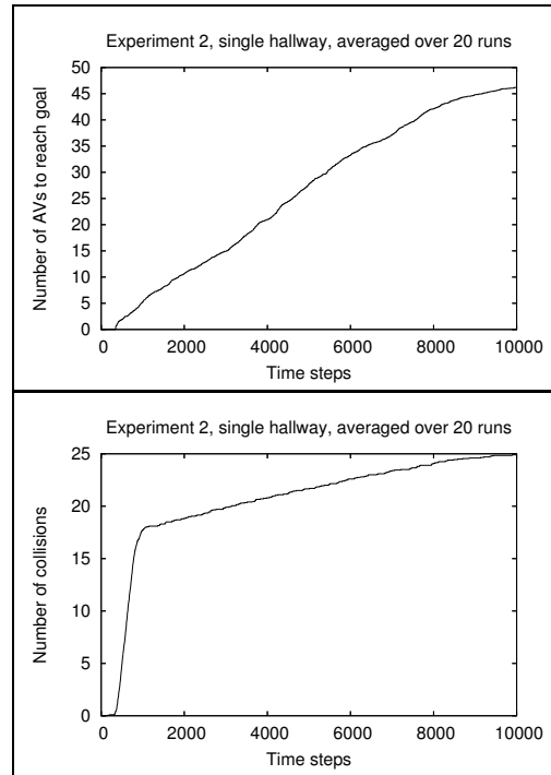
Fig. 5. Here we show the graphs for our first set of SSS experiments. We had hoped that having one dominant AV would break up deadlocks around the hallway entrance, but this did not occur. Notice that there is not a big difference between the top graph here and the graph in Figure 4.
